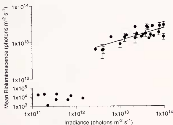
Figure 7. Effect of light intensity on average maximum bioluminescence produced by Sergestes similis . All stimuli were at a wavelength of 490 nm. The magnitude of bioluminescence measured during the last 20 s of each 60-s test stimulus was averaged for each individual. Ten specimens were tested; means \pm SE are shown. Responses for stimulus irradiance > 2 \times 10^{12} photons \text{m}^{-2} \text{s}^{-1} were best described by the power law (log-log) equation y = (1.87 \times 10^6)x^{0.35} ( r^2 = 0.61 ). At lower stimulus irradiance values, light levels were near background. Note the separate scale for above-threshold bioluminescence.
